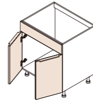
Item: Vanity Sink Base With 2 Doors+1 Fake Drawer Code: VSB24, VSB27, VSB30, VSB36 HxD: 30" x 21"
